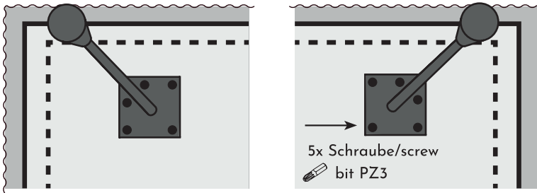
Unteransicht in Detail Bottom view detail
